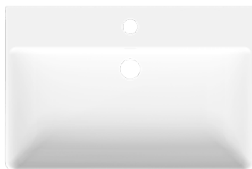
U079 700 × 465 × 95 (660 × 290 × 95)
